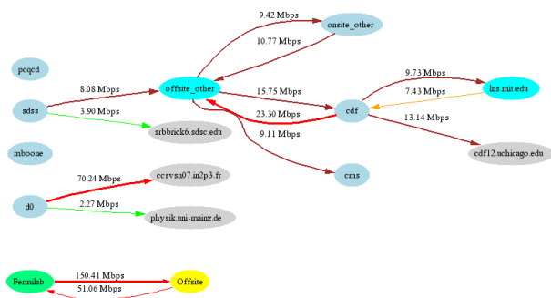
Figure 5: Example of adjusted mapper's graphs.
