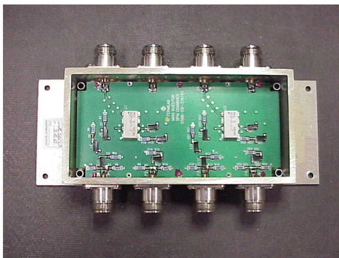
Figure 1: Combiner Module
